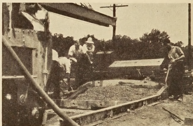
FIGURE 4.—FINISHER SPREADING CONCRETE
